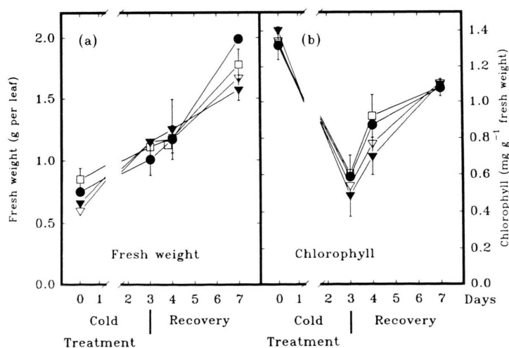
Fig. 1. Influence of cold treatments and fumigation with automobile exhaust and O 3 on the total fresh weight (a) and the Chl content (b) of primary leaves of cucumber plants during 7 days following a first 2-h cold exposure to 0–4 °C in light of 12-day-old plants. Cold exposures were repeated three times, once per day on days 1–3, and the plants then allowed to recover for an additional 4 days. Fumigation conditions: □ filtered air; ● automobile exhaust; ▼ automobile exhaust + O 3 ; ▽ O 3 . At day 0, plants had been previously fumigated for 4 days.
