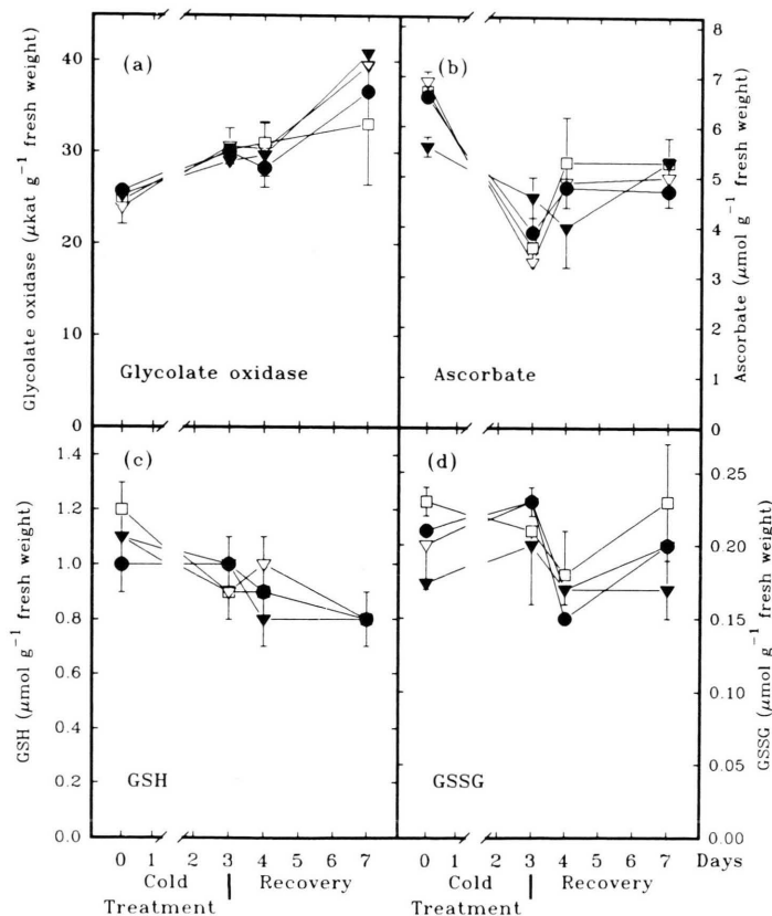
Fig. 4. Influence of cold treatments and fumigation with automobile exhaust and \text{O}_3 on the activity of glycolate oxidase (a) and the contents of reduced ascorbic acid (b), reduced glutathione (c) and oxidized glutathione (d) in primary leaves of cucumber during 7 days following a first 2-h cold exposure to 0–4 °C in light of 12-day-old plants. Cold exposures were repeated three times, once per day on days 1–3, and the plants then allowed to recover for an additional 4 days. Fumigation conditions: □ filtered air; ● automobile exhaust; ▼ automobile exhaust + \text{O}_3 ; ▽ \text{O}_3 . At day 0, plants had been previously fumigated for 4 days.
